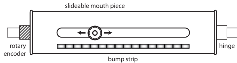
Fig. 3.10 – A schematic of the Jamboxx (Whalen, Luther, and DiCesare 2011).
